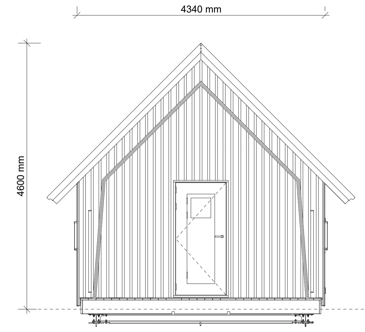
Front elevation
