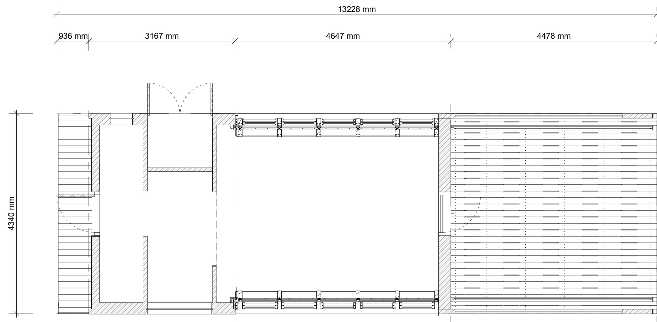
Floor plan – Ground floor
