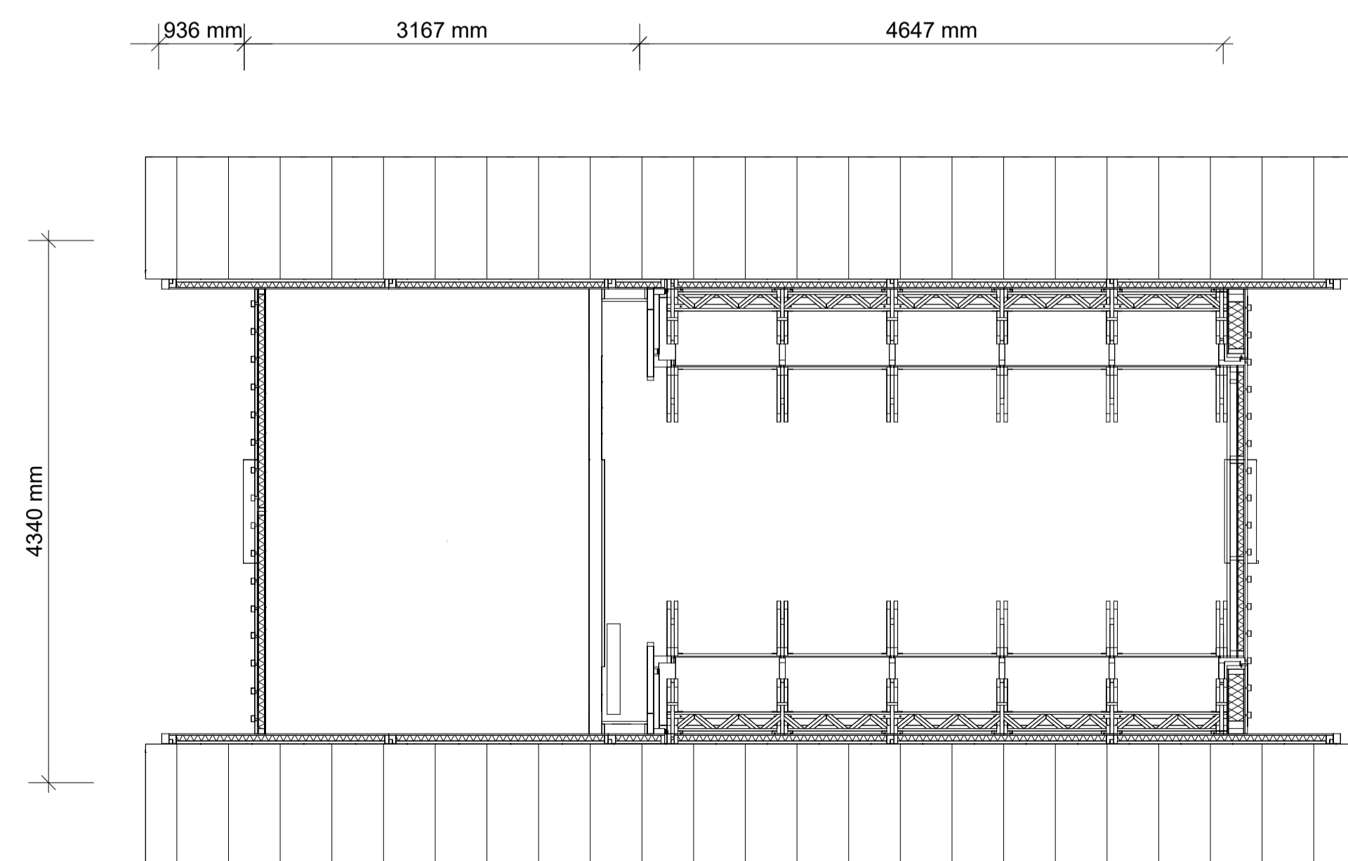
Floor plan – Mezzanine
