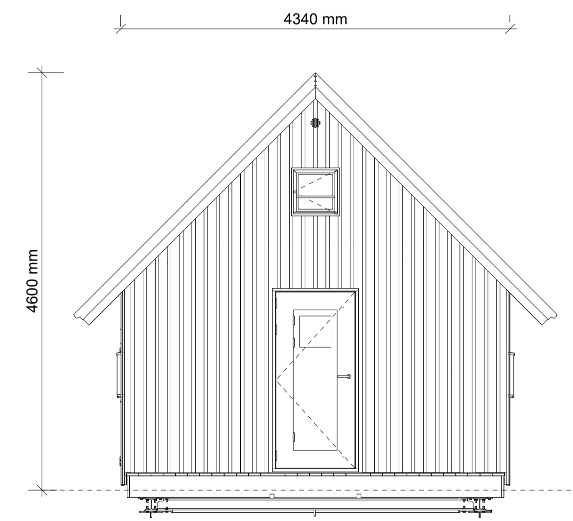
Back elevation
